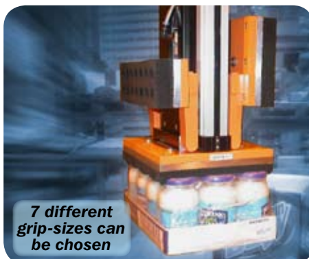
UniGripper WingGripper for picking of single SKU's into mixed pallets.
